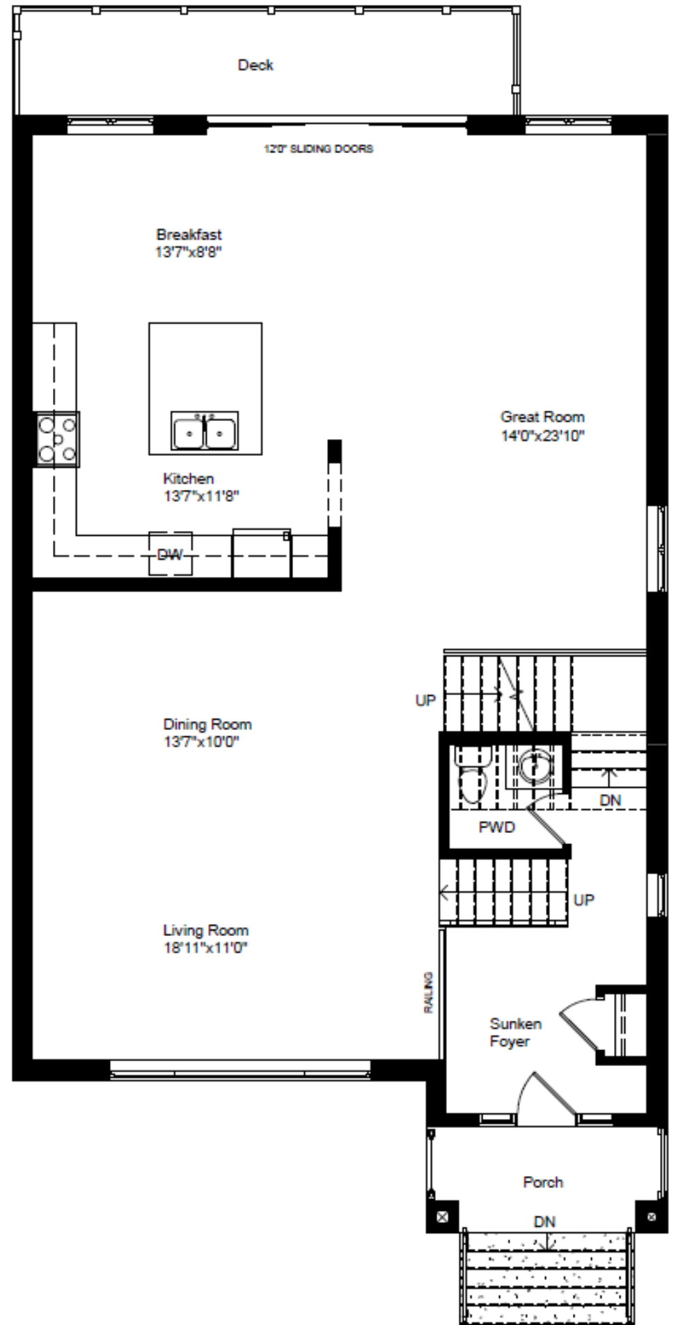
MAIN FLOOR PLAN OPTIONAL GREAT ROOM ENLARGED
