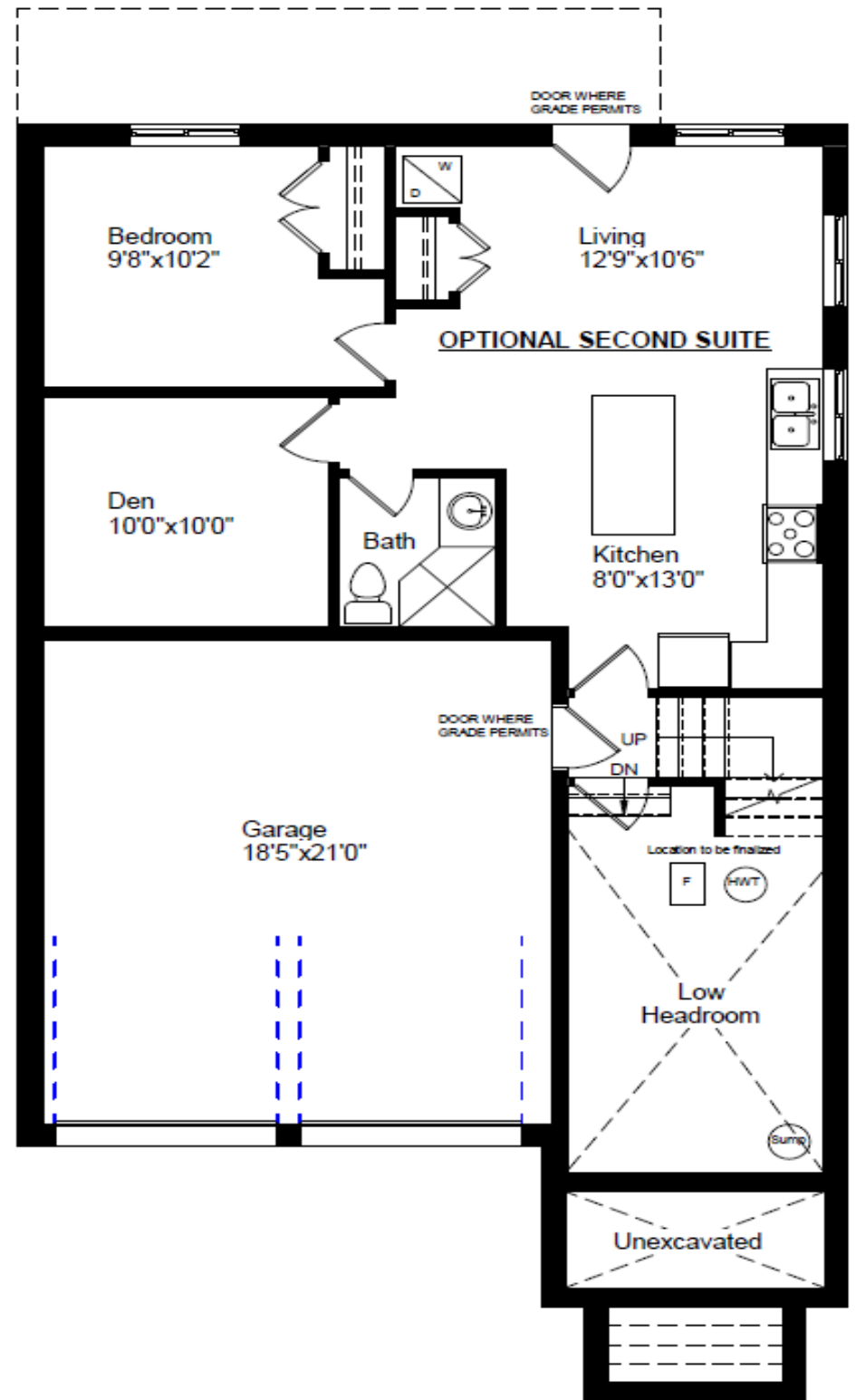
BASEMENT FLOOR PLAN OPTIONAL SECOND SUITE
