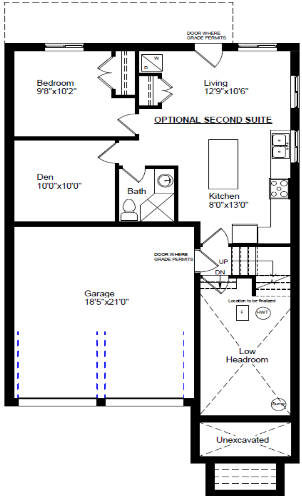
BASEMENT FLOOR PLAN OPTIONAL SECOND SUITE
