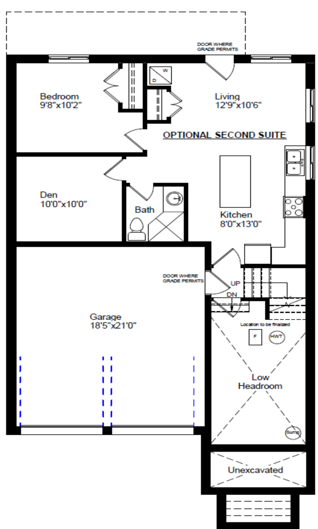
BASEMENT FLOOR PLAN OPTIONAL SECOND SUITE
